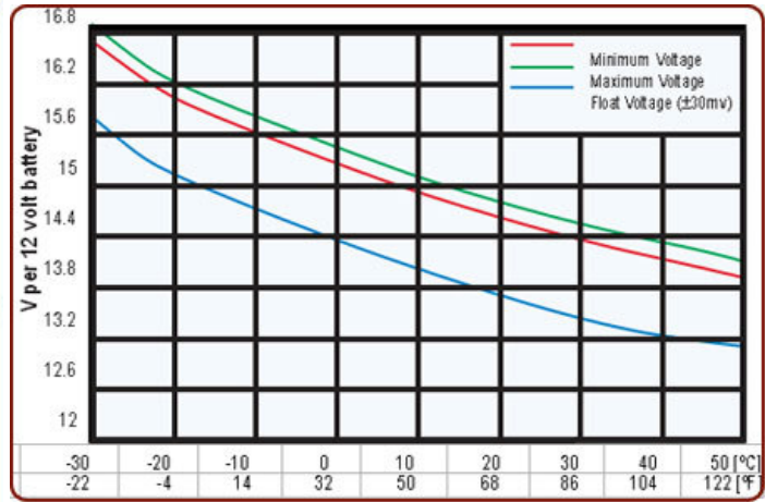
Constant Charging Voltage Vs Temp
