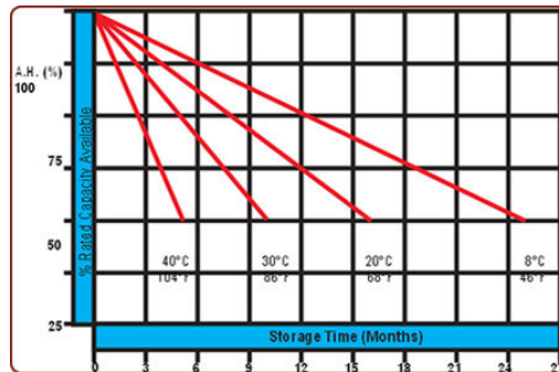
Self Discharge Vs Temp. Curve
