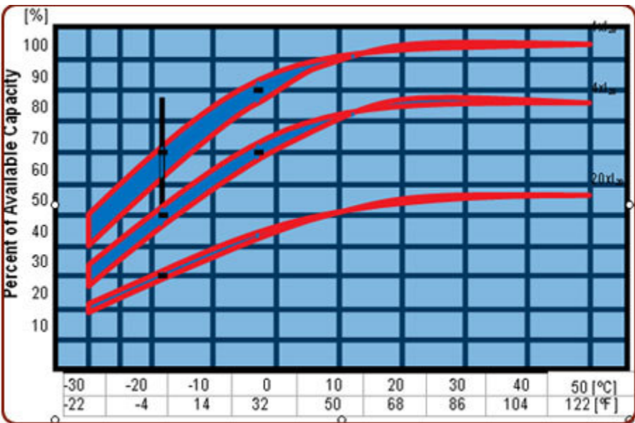
Capacity Vs Operating Temp
