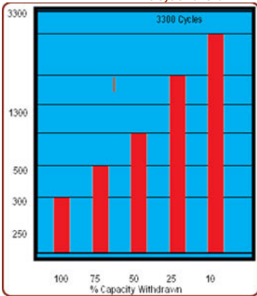
No.ofCyclesVs.DOD at+25°C(77°F) discharge with C 20 Discharge Rate
